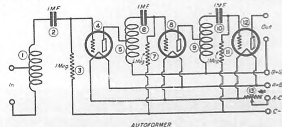
AUTOTRANSFORMER
